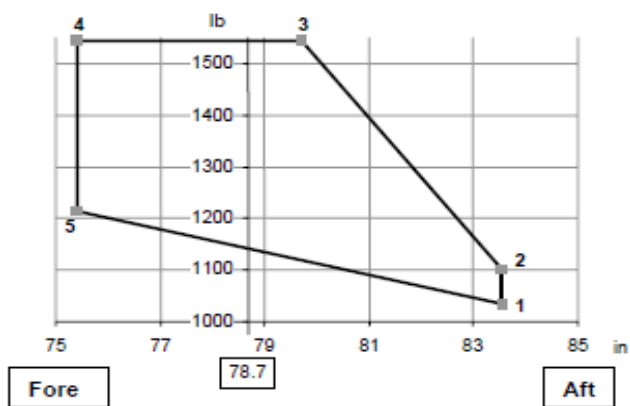
Longitudinal Weight and Balance diagram
